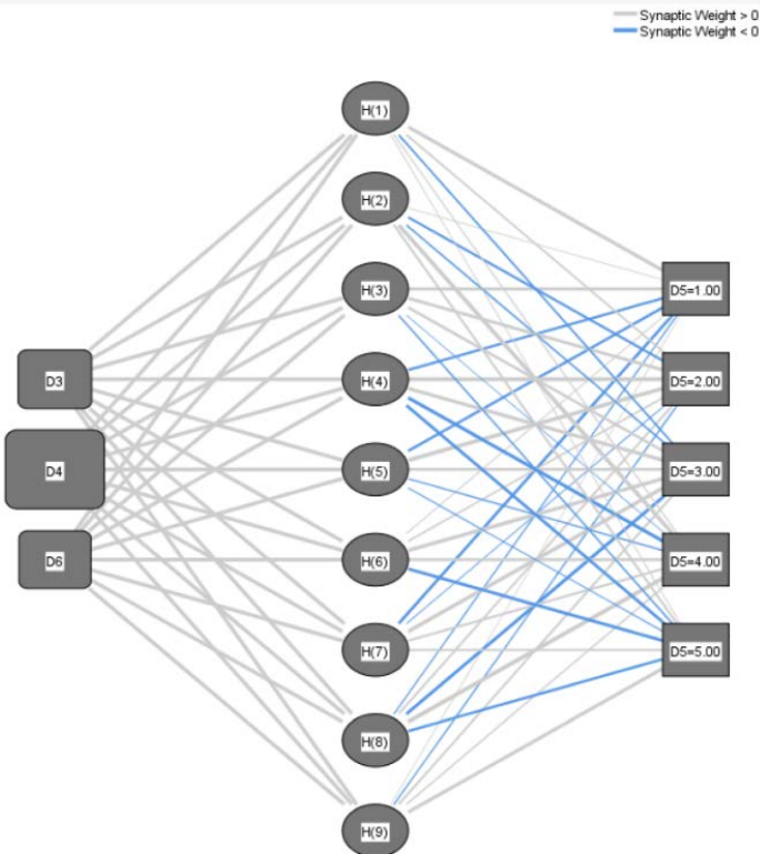
Figure 2. RBF architecture.
